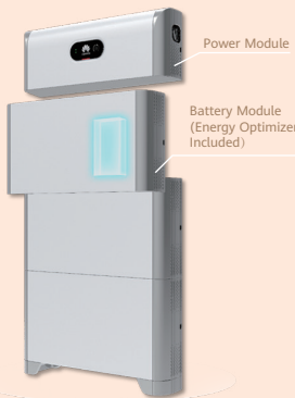
LUNA2000-5/10/15-50 String Battery Solution
