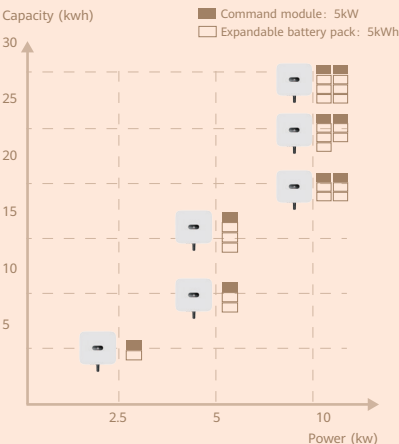
LUNA2000-5/10/15-50 String Battery Solution
