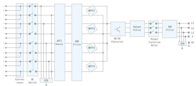
Circuit Diagram
