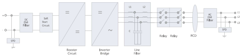
LUNA2000-213KTL-H0
