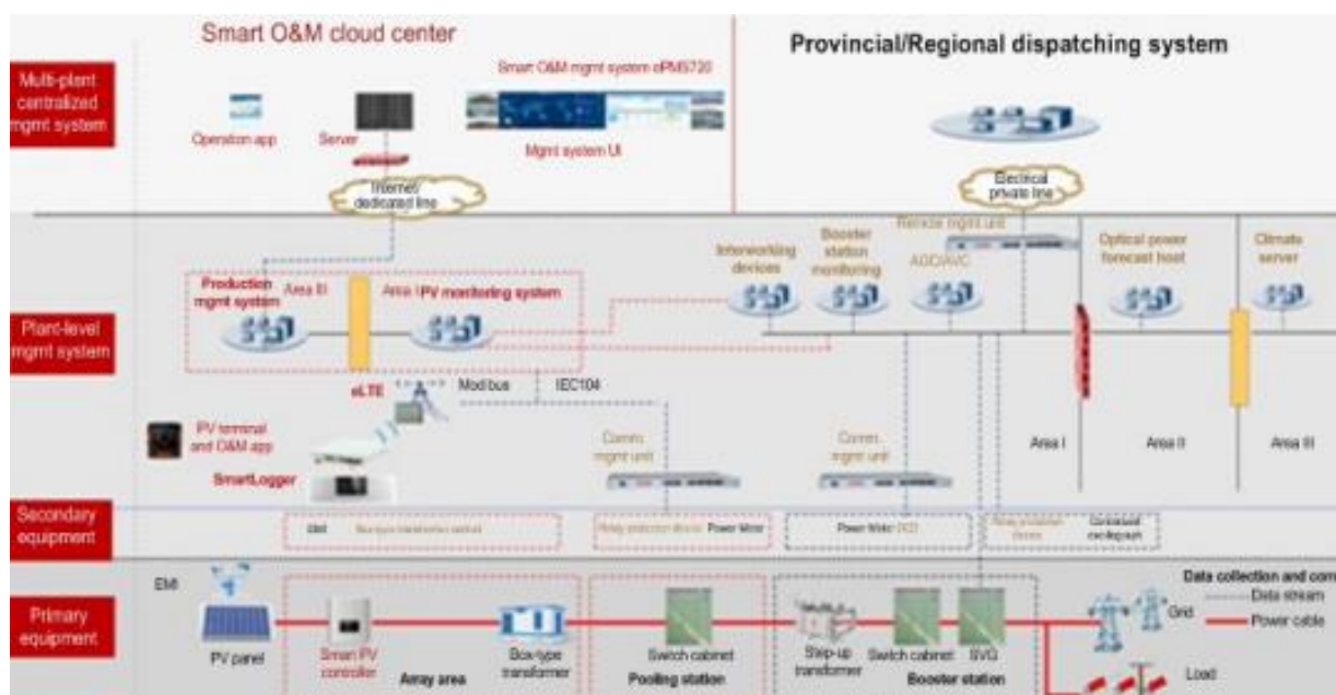
C&I Inverter Solution Architecture
