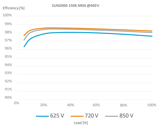
Efficiency Curve
