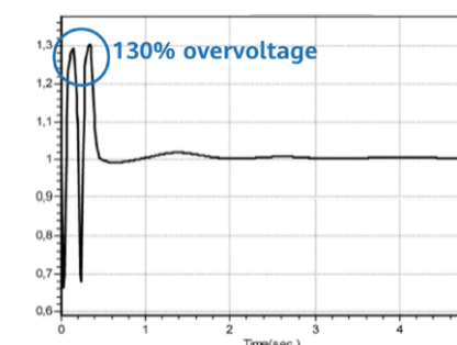
Figure 1 Overvoltage caused by continuous commutation failure in the Jarud Banner 500 kV project
