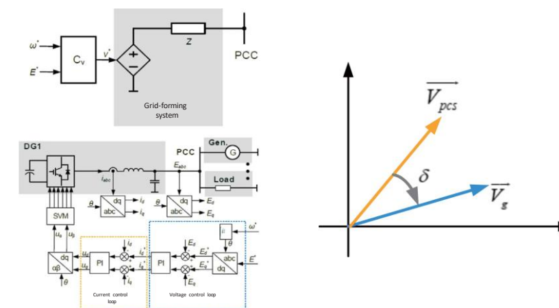
Figure 7 Basic control diagram of grid forming technologies
