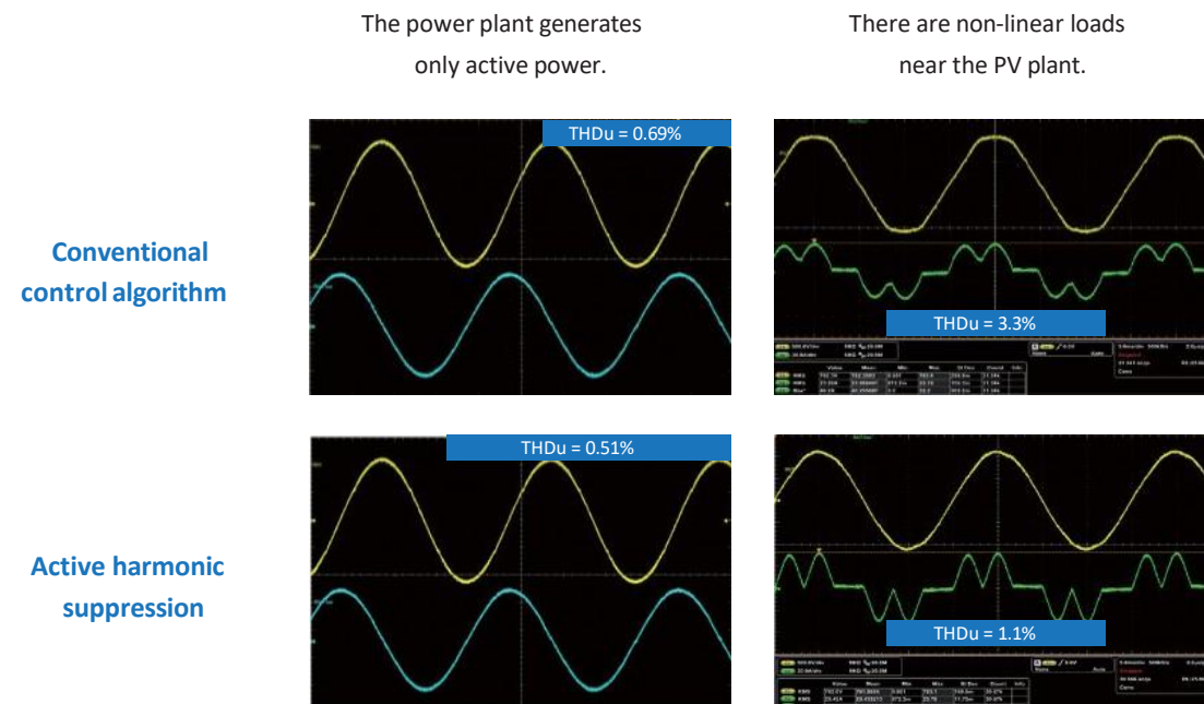
Figure 18 Comparison between the active harmonic suppression technology and the conventional solution
