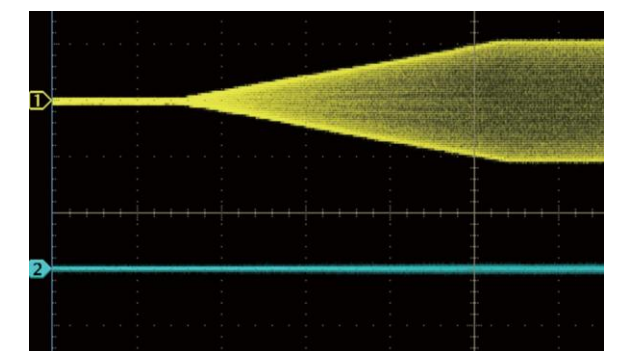
Figure 17 Huawei solution minimizes circulating current
