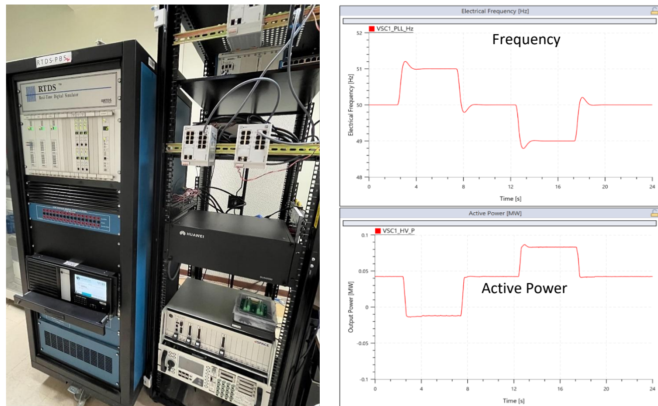
Figure 19 RTDS test bench in Dammam and test results of RoCoF and synthetic inertia + primary frequency response
