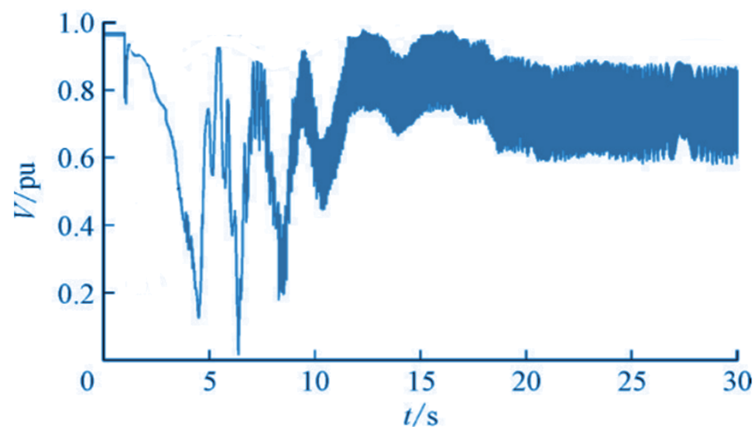
Figure 3 Voltage instability caused by an N-2 fault on a 750 kV transmission line in Haixi
