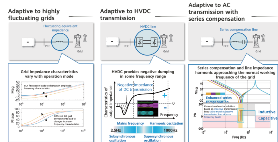
Figure 13 Adaptive virtual impedance technology
