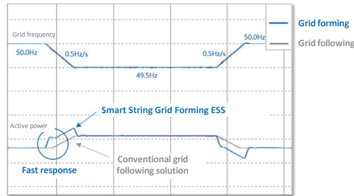
Figure 11 Frequency response capability comparison between the Smart String Grid Forming ESS and the conventional PV+ESS system
