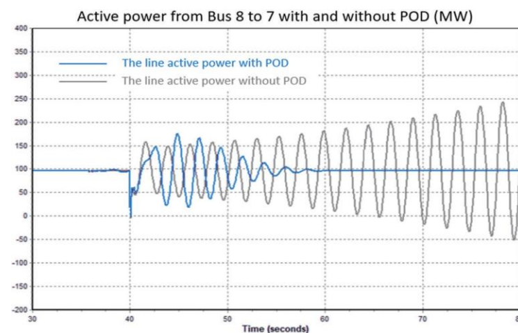
Figure 12 Power suppression effect of low-frequency POD
