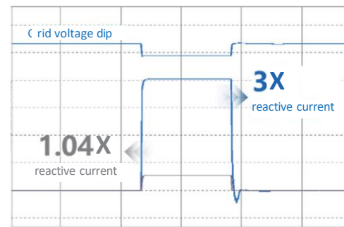
Figure 09 High-current transient support of the Smart String Grid Forming ESS
