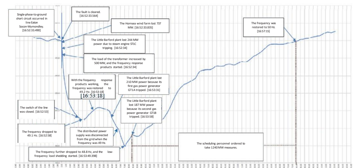
Figure 4 Timing and frequency changes during the power outage on August 9 in the UK
