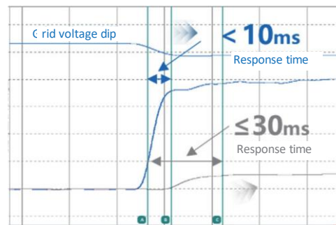
Figure 8 Fast reactive current response of the Smart String Grid Forming ESS
