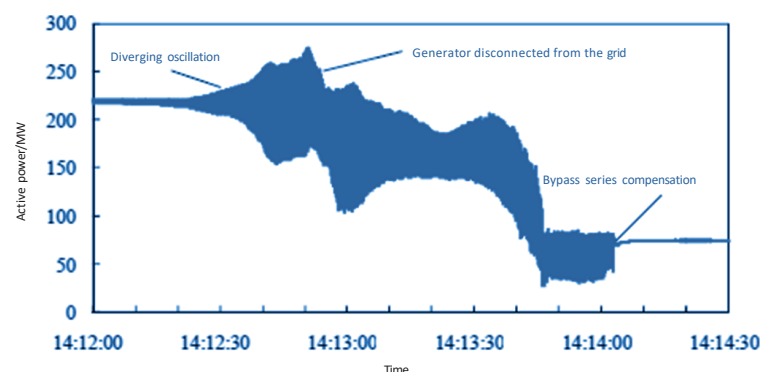
Figure 5 Power oscillation of a wind farm in Guyuan, Hebei
