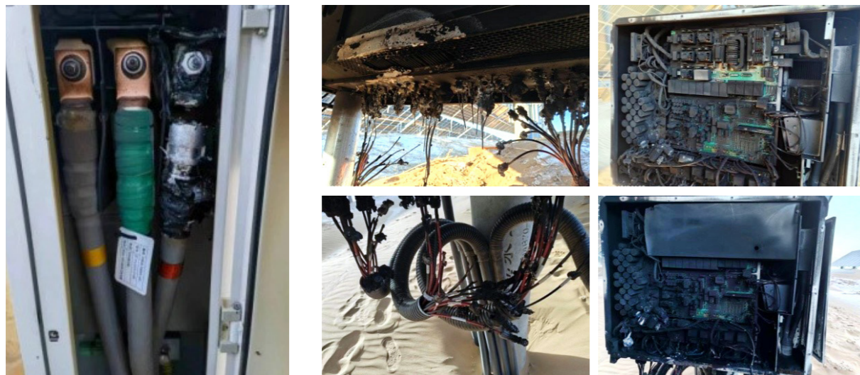
> Burnt terminals
