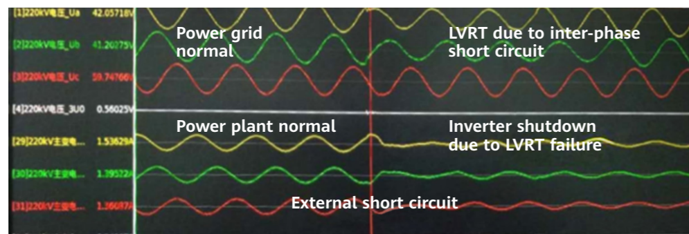
> LVRT waveforms
