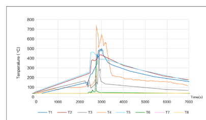
Figure 54 Cell temperature changes
