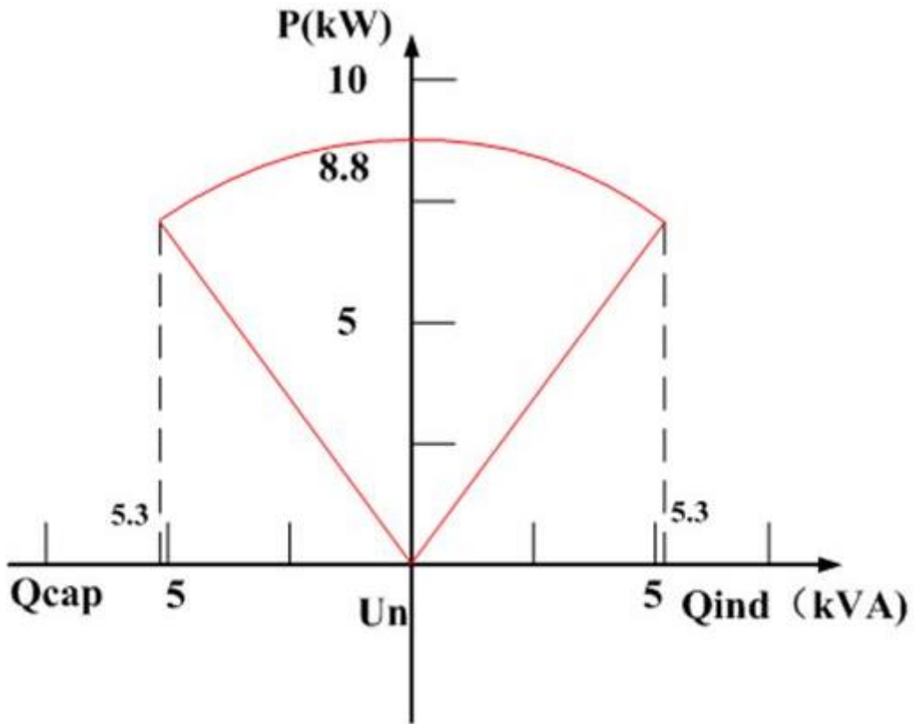
SUN2000-8kTL PQ Curve
